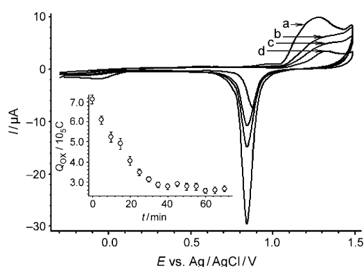
Figure 2. Cyclic voltammograms ( 50 \text{ mVs}^{-1} ) of Au recorded in 0.1 \text{ M H}_2\text{SO}_4 after exposure to \text{OH}^\bullet for a) 0, b) 10, c) 15, and d) 70 min. Inset: Charge of the oxidation peak versus time of reaction with \text{OH}^\bullet .
