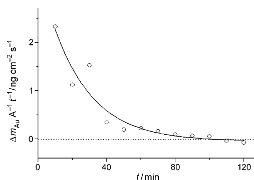
Figure 3. Rate of Au dissolution as function of time. A gold plate with 4.2 \text{ cm}^2 overall geometric surface area was exposed to 2 \text{ mL} of Fenton's reagent. Every 10 \text{ min} , 300 \mu\text{L} solution was removed for analysis and replaced by 300 \mu\text{L} 1 \text{ M H}_2\text{O}_2 solution.
